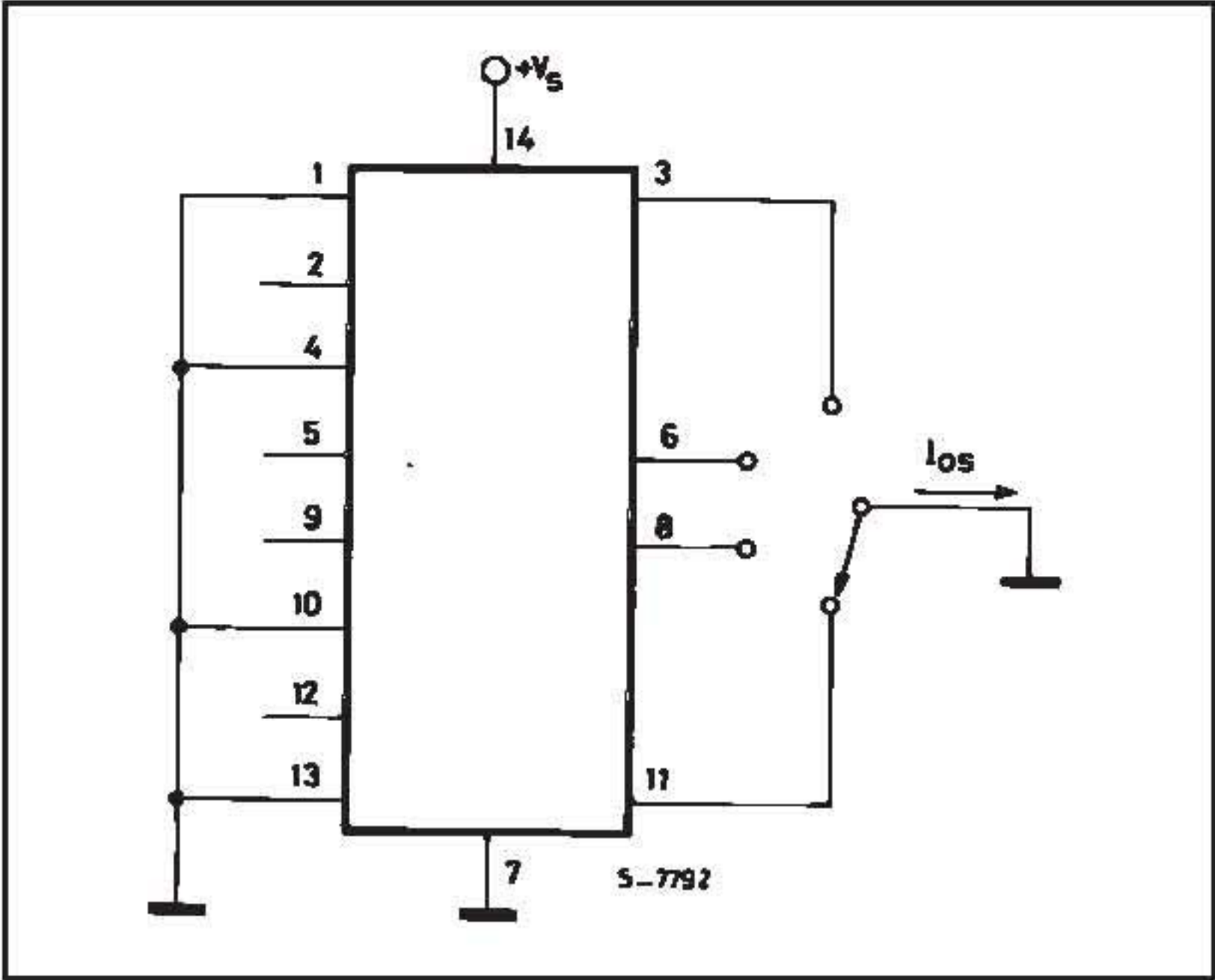
Figure 4 :Output Short-Circuit Current
