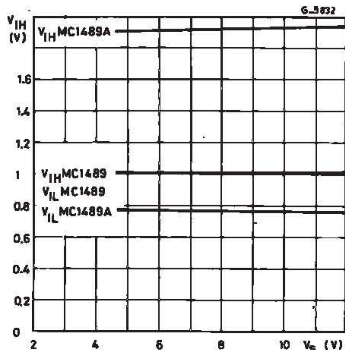
Figure 11 :Input Threshold versus Power Supply Voltage
