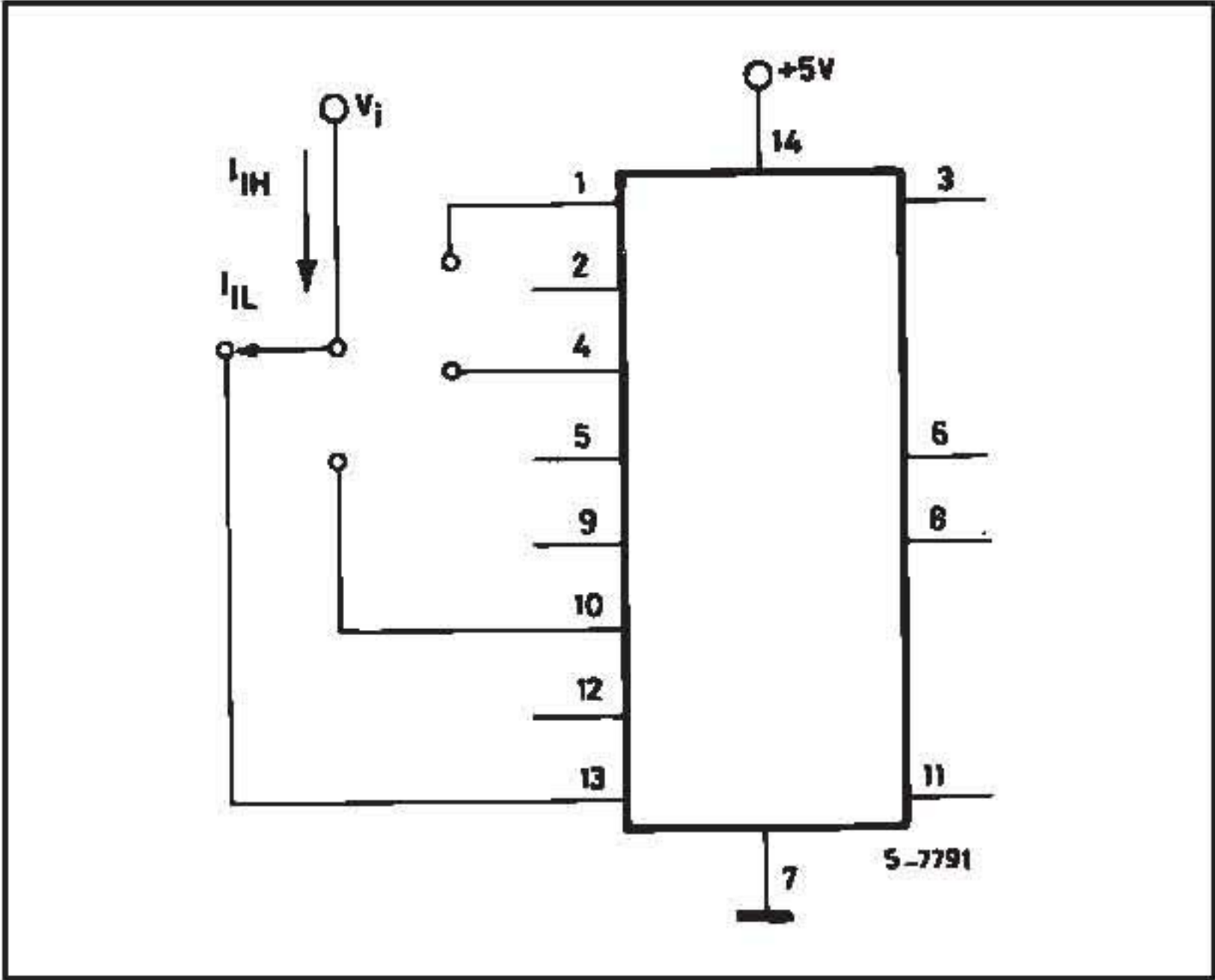
Figure 3 :Input Current
