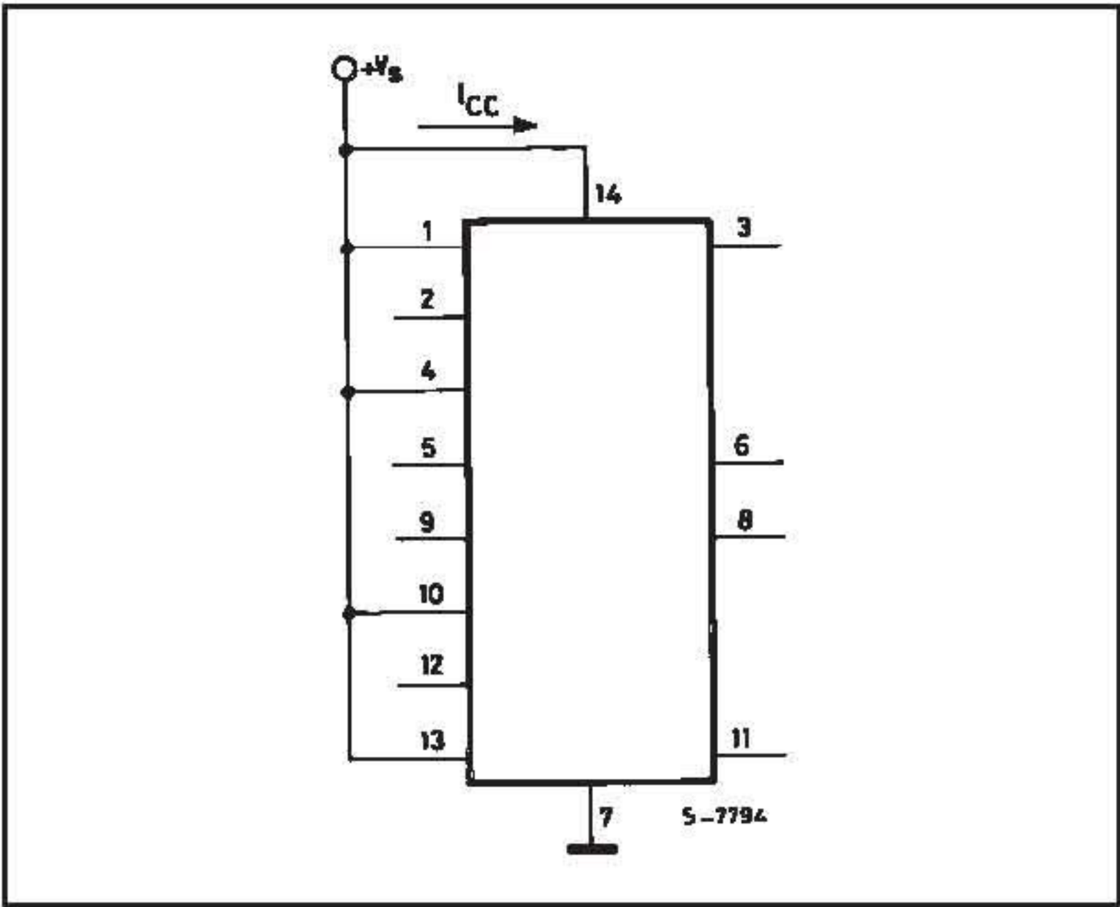
Figure 6 :Power Supply Current
